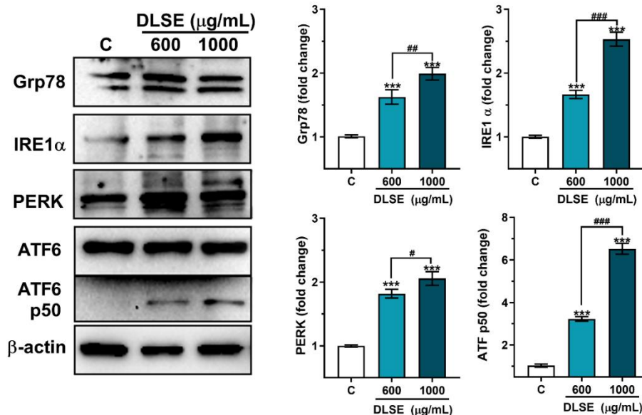
Figure 5. Effects of Dicentrarchus labrax scale extract (DLSE) on endoplasmic reticulum (ER) stress-related proteins in glioblastoma cells. U-87MG cells were treated with DLSE (600 and 1000 μg/mL) for 72-h. Protein levels of Grp78, IRE1α, PERK, and ATF6 (full-length and cleaved ATF6 p50) were analyzed by Western blotting (n=3). β-actin was used as a loading control. Data are expressed as mean±SD. *** p < 0.001 versus vehicle control; ### p < 0.001, ## p < 0.01, # p < 0.05 indicate comparison between different groups. Statistical comparisons were performed using one-way ANOVA followed by Tukey's post hoc test.
